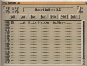
VirusZ has a comprehensive boot block laboratory...
